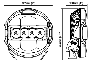
IDL0901S Op. Volt: 10-32V DC
