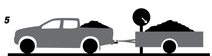
5 Total weight of vehicle plus trailer weight = GCM (gross combined mass) Ensure total weight of vehicle and trailer does not exceed manufacturers GCM
