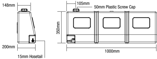
IWT006 - 50L TAPERED TANK
