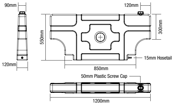
IWT005 - 50L WHEEL ARCH TANK
