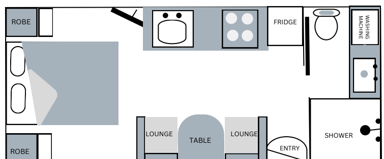
IRV196 REAR DOOR LAYOUT
