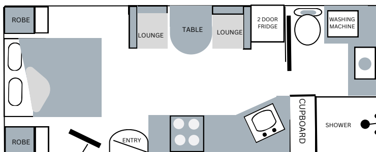
IRV216LE ANGLED KITCHEN LAYOUT
