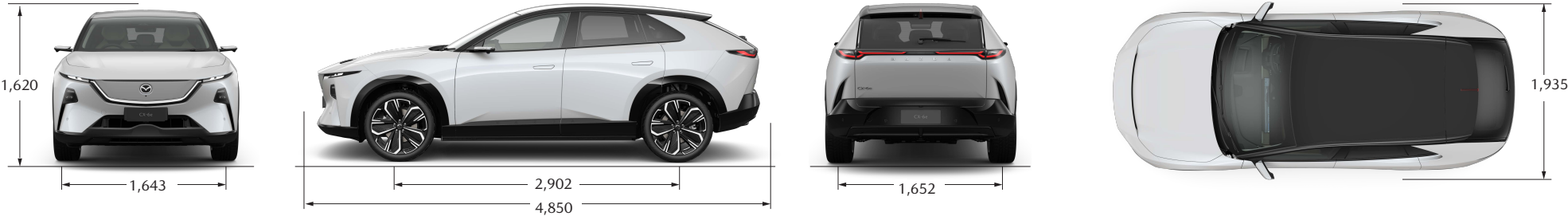
DIMENSIONS (mm)
