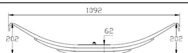
032900 THREE LEAF HIGH ARCH 4990kg RATING, WEIGHT 24kg
