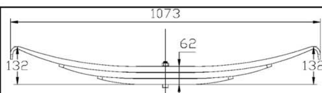
033500 THREE LEAF LOW ARCH 4990kg RATING, WEIGHT 24kg
