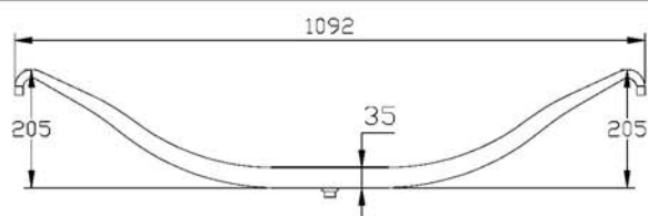
033100 MONO LEAF HIGH ARCH 4990kg RATING, WEIGHT 17kg
