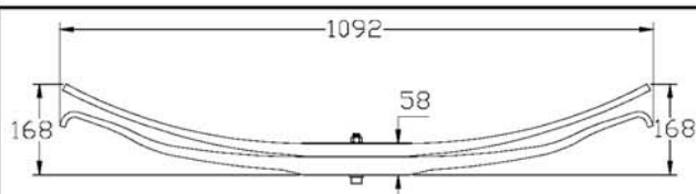
160102 TWO LEAF LOW ARCH 4990kg RATING, WEIGHT 24kg
