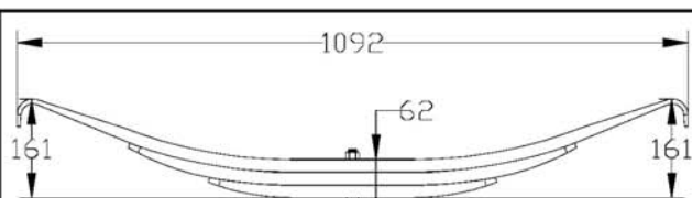
069400 THREE LEAF MED ARCH 4990kg RATING, WEIGHT 24kg
