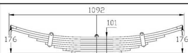
017806 EIGHT LEAF MED ARCH 4990kg RATING, WEIGHT 43kg
