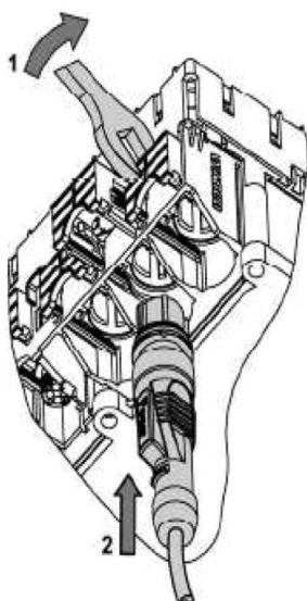
Above: WABCO TEBS E Modulator Plugs and dismantling of cables and protective caps.
